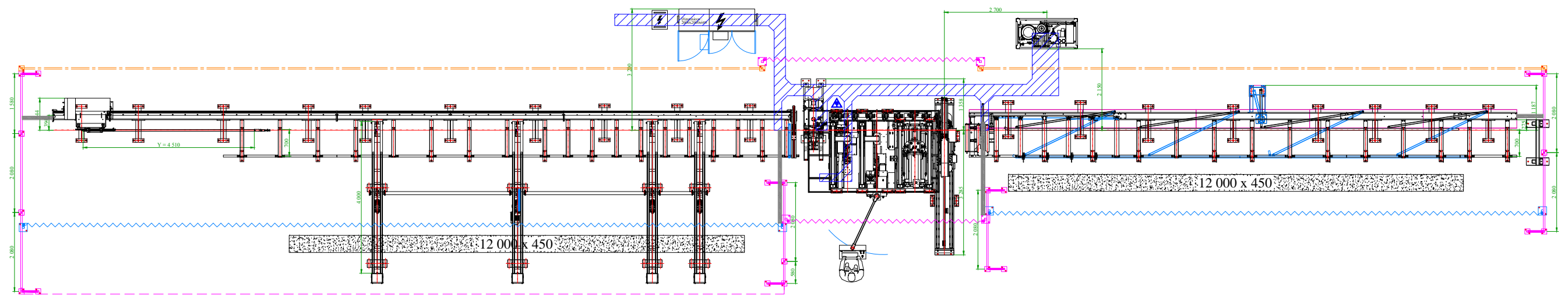
LIGNE MAPS 456 LINE FRONT VIEW
